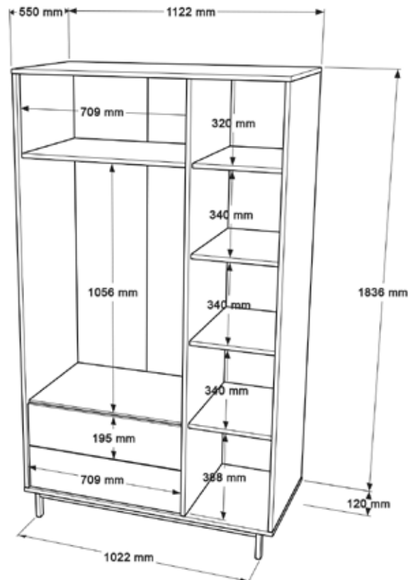
TECHNICAL DRAWING
