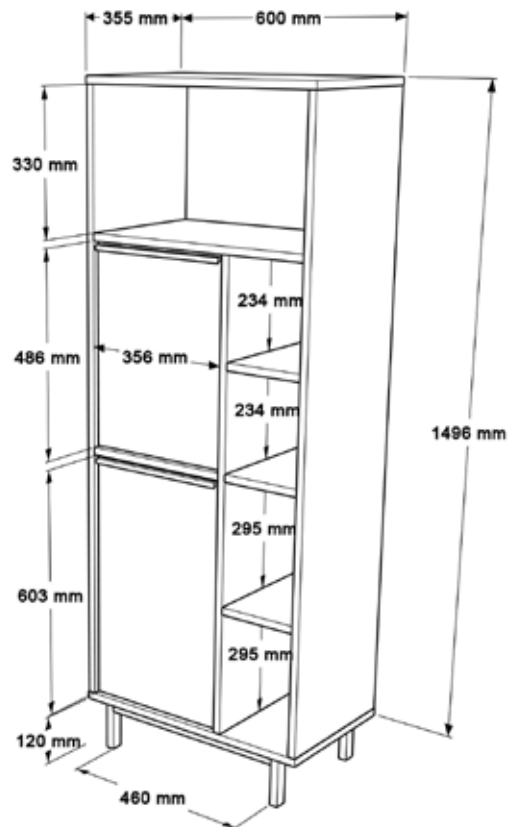
TECHNICAL DRAWING
