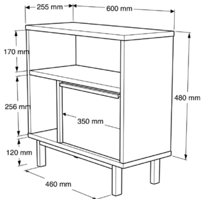
TECHNICAL DRAWING
