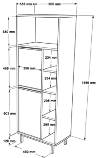
TECHNICAL DRAWING
