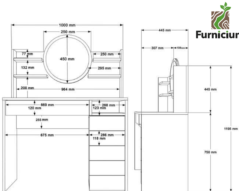
TECHNICAL DRAWING
