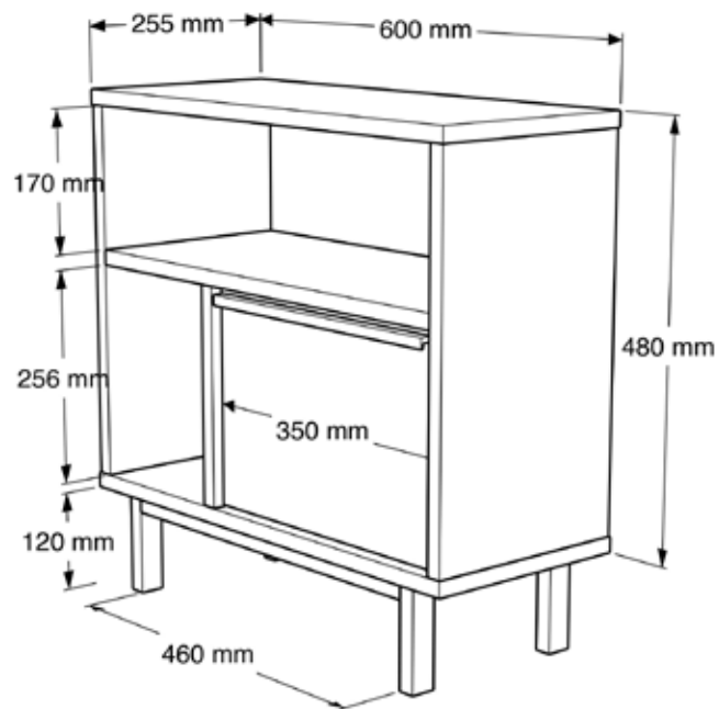
TECHNICAL DRAWING
