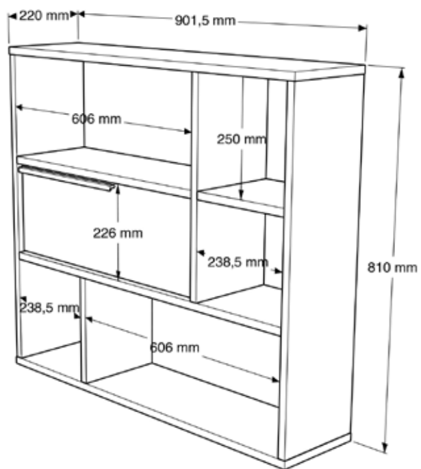
TECHNICAL DRAWING
