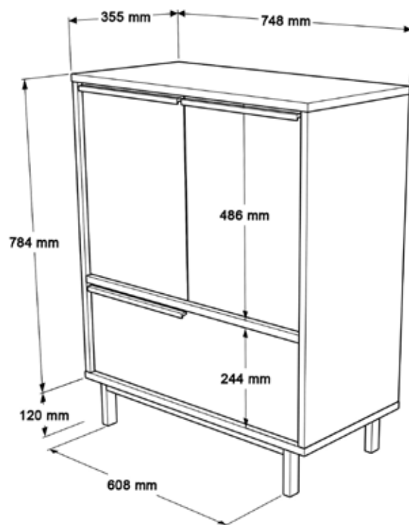
TECHNICAL DRAWING
