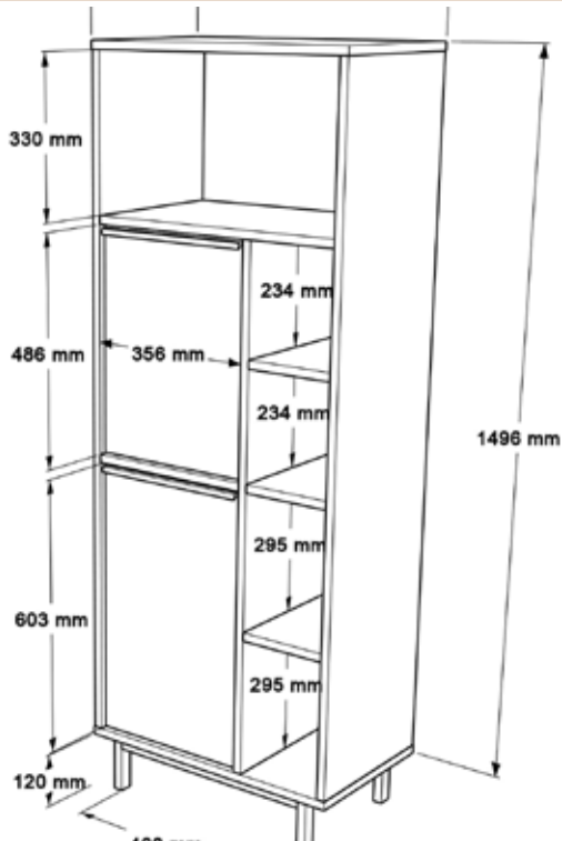
TECHNICAL DRAWING
