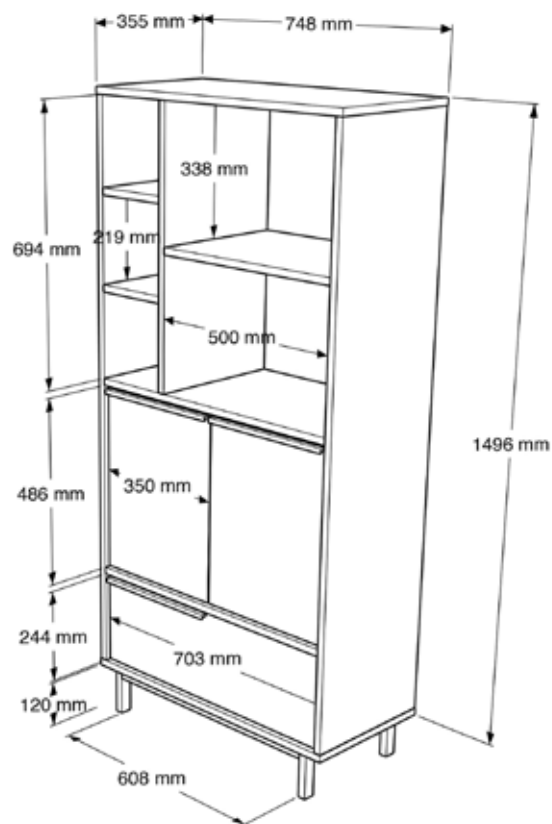
TECHNICAL DRAWING
