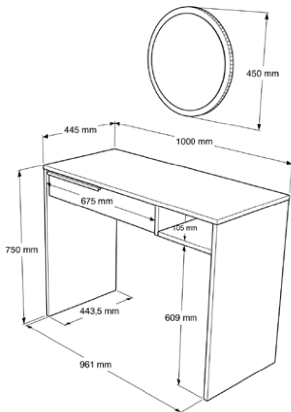
TECHNICAL DRAWING
