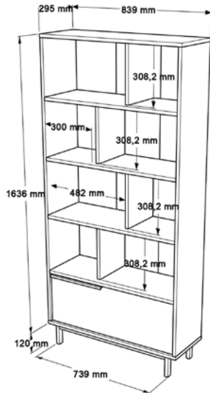
TECHNICAL DRAWING
