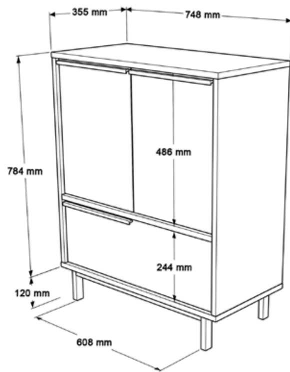
TECHNICAL DRAWING
