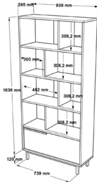
TECHNICAL DRAWING
