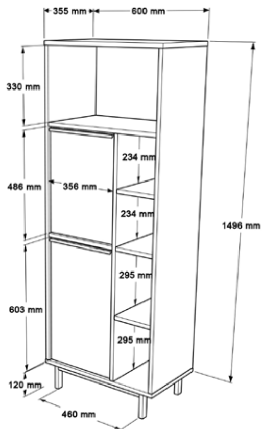
TECHNICAL DRAWING
