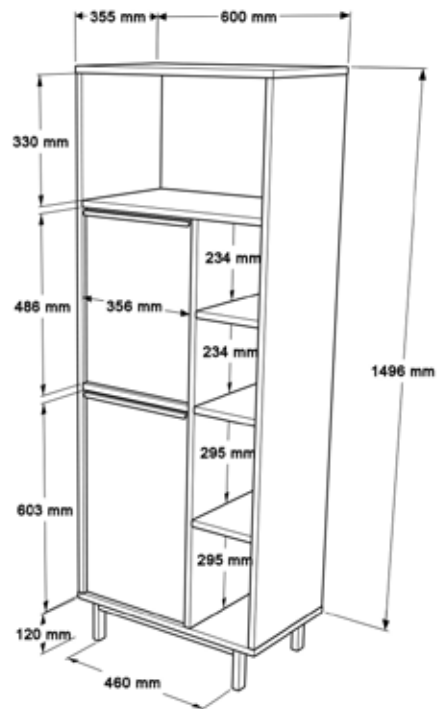
TECHNICAL DRAWING
