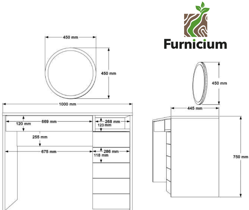
TECHNICAL DRAWING
