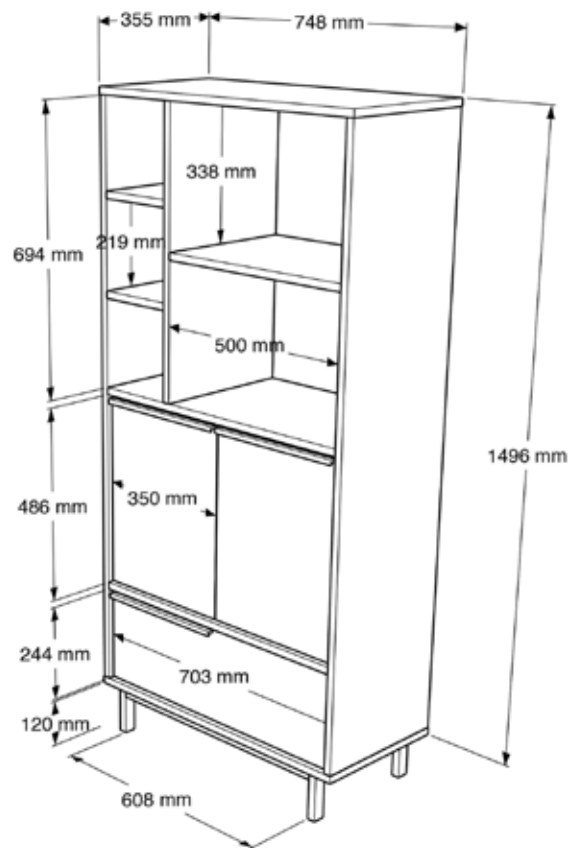
TECHNICAL DRAWING
