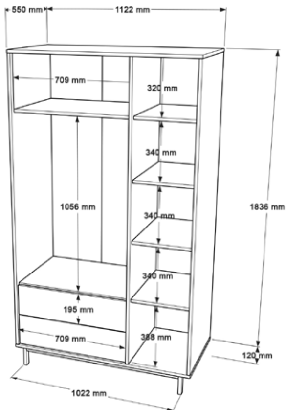
TECHNICAL DRAWING
